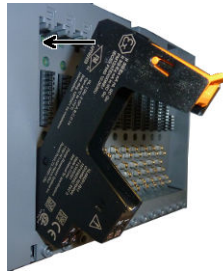
Figure 2-5: CHARM Terminal Block installation
